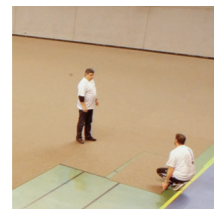
PROTECTILES Textile protection tiles 1 box of 5 pcs - 10m 2 total weight: 3.1kg/m 2 total thickness: 5.2 mm 1 m x 2 m
